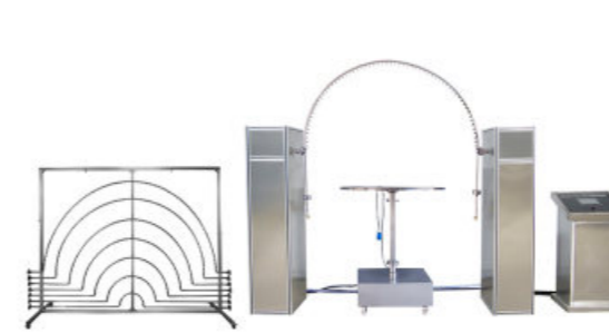
RNH34 (IPX3X4 Test Equipment)
